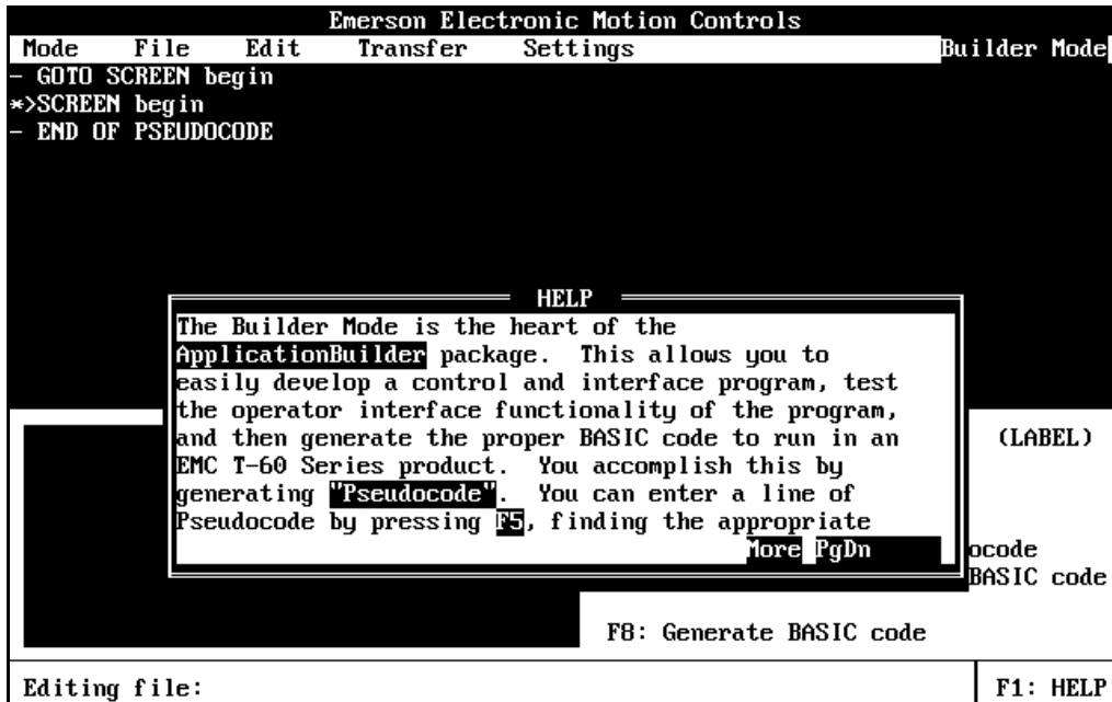
Figure 1 Help Screen
